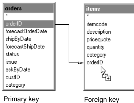
Figure 8-10 Creating a join manually
