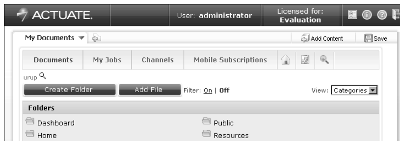
Figure 2-10 Tabbed skin
