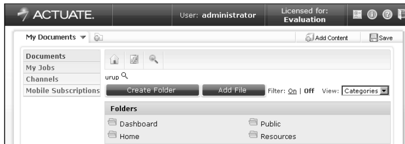
Figure 2-9 Classic skin
