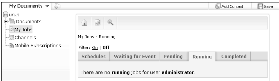
Figure 6-14 Running page
