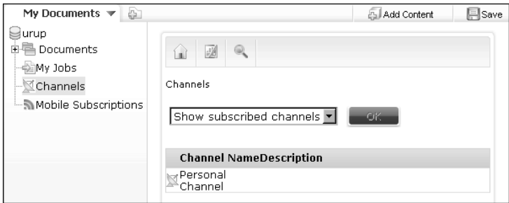
Figure 6-2 Channels page
