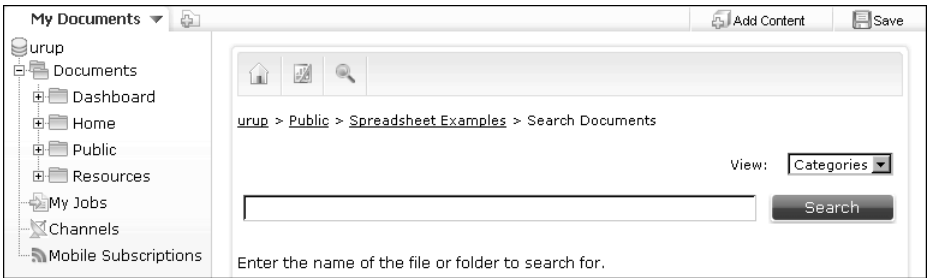
Figure 6-17 Search results
