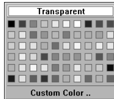
Figure 8-15 Color selector
