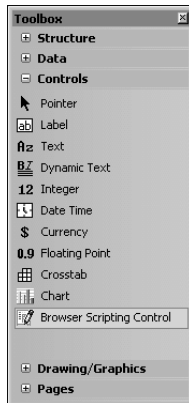
Figure 26-1 Controls toolbox
