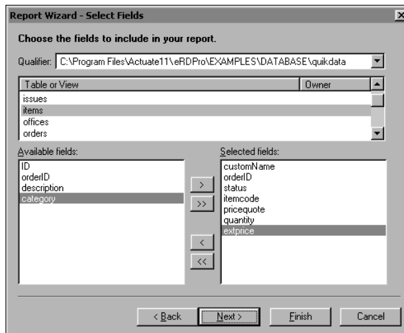
Figure 1-14 Select Fields
