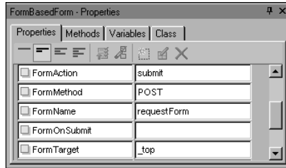
Figure 26-7 DHTMLForm properties
