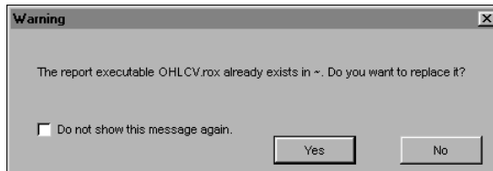
Figure 22-3 Warning message
