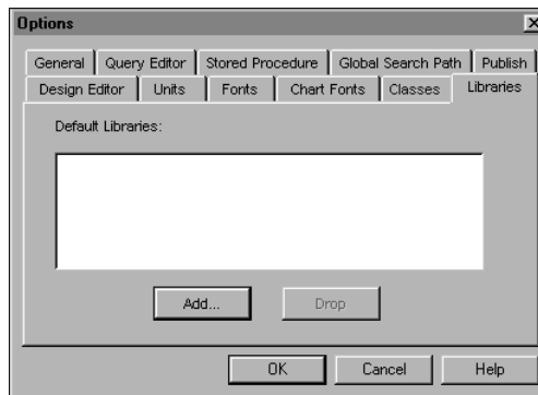
Figure 21-15 Options—Libraries
