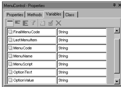
Figure 26-8 DHTMLMenuControl variables
