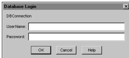
Figure 1-13 Database login
