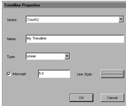
Figure 8-35 Trendline Properties
