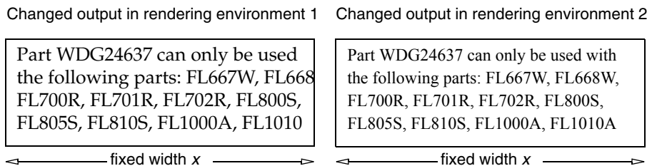
Figure 11-11 Reducing LineWidthPadding
