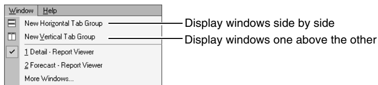
Figure 29-13 Window menu
