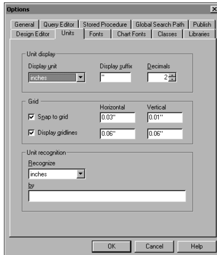
Figure 1-8 Options—Units
