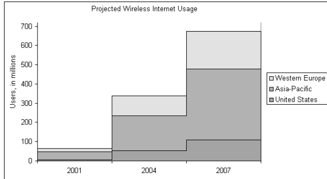
Figure 7-12 Step chart
