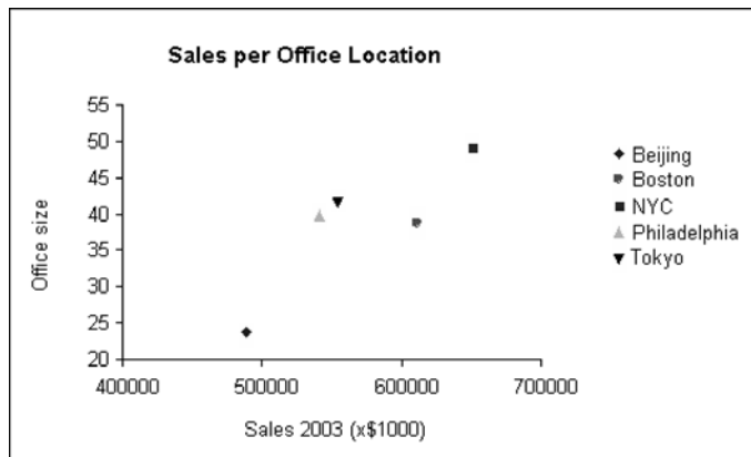
Figure 7-19 Scatter chart
