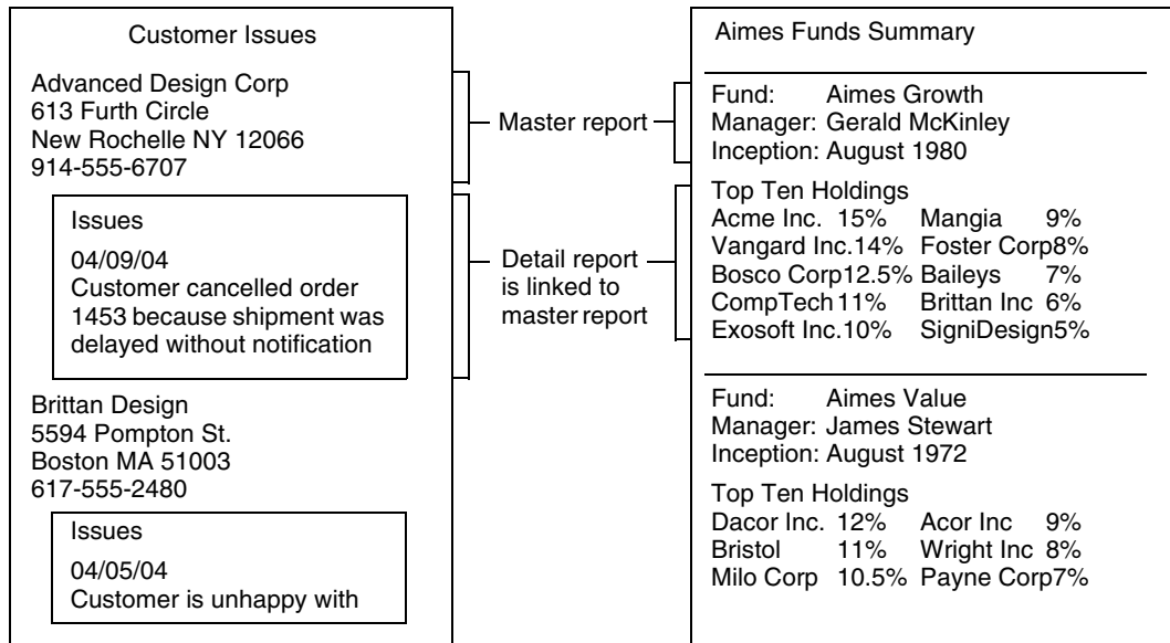
Figure 13-24 Linked subreports
