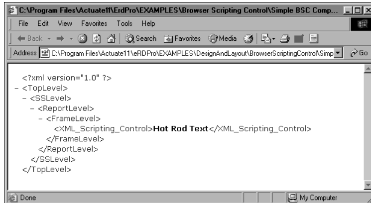
Figure 27-2 XML file
