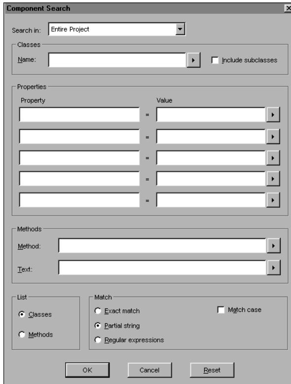
Figure 2-21 Component Search
