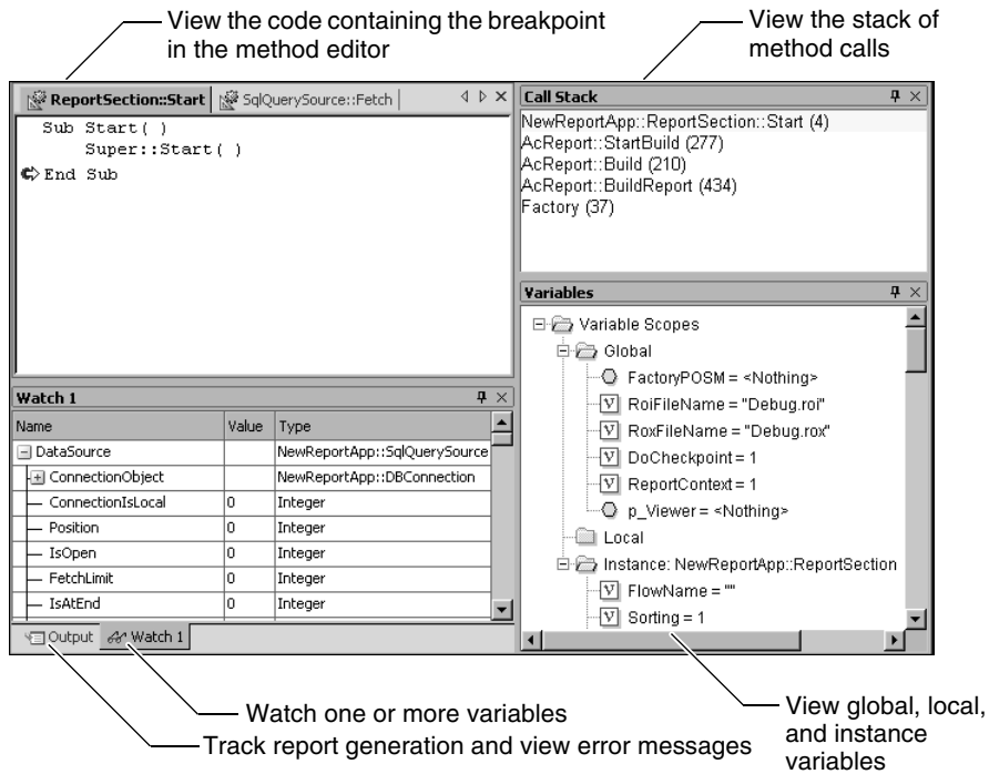
Figure 16-1 Debug perspective
