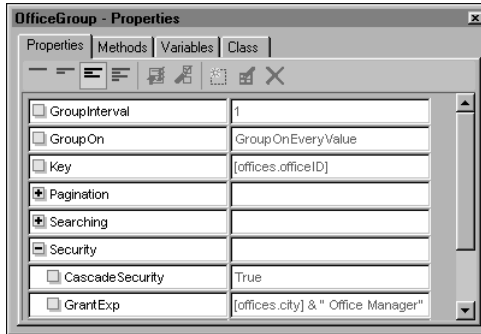
Figure 18-5 OfficeGroup—Properties
