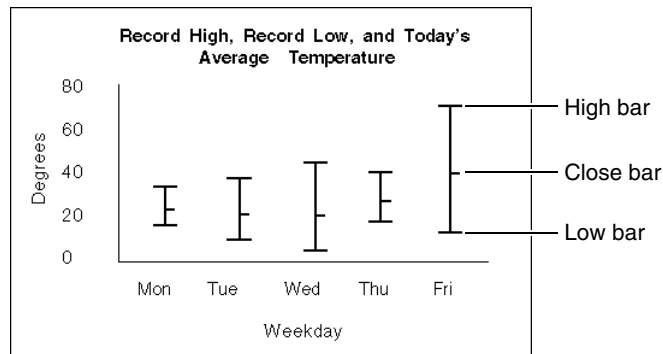
Figure 7-13 Stock charts
