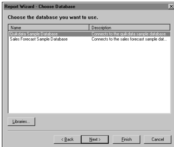
Figure 1-12 Database connections
