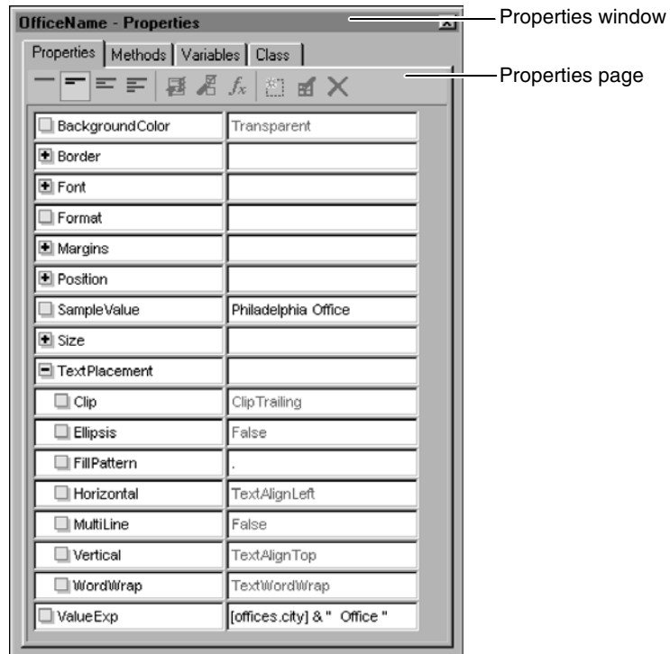
Figure 5-3 Properties window
