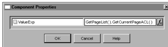
Figure 18-6 Component Properties—ValueExp
