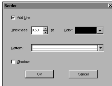
Figure 8-16 Border setup
