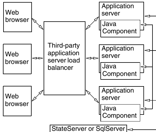
Figure 1-1 Load-balancing architecture for Java Component
