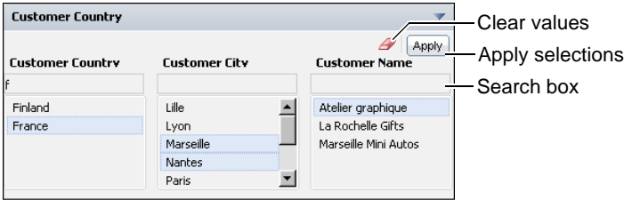
Figure 4-134 Displaying a selector group in horizontal lists
