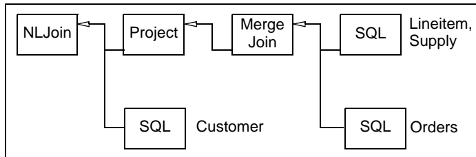
Figure 7-1 Example of part of the query plan for which values for the map and join column properties have been provided
