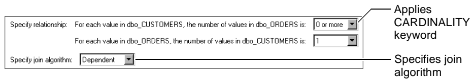
Figure 5-21 Optimizing a join
