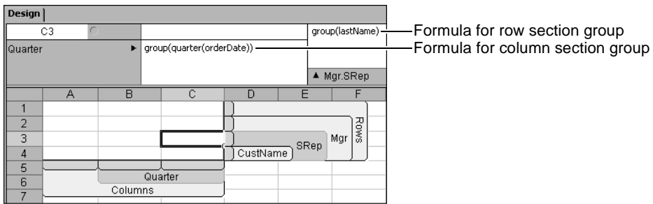
Figure 7-10 Examining the group keys for row and column sections
