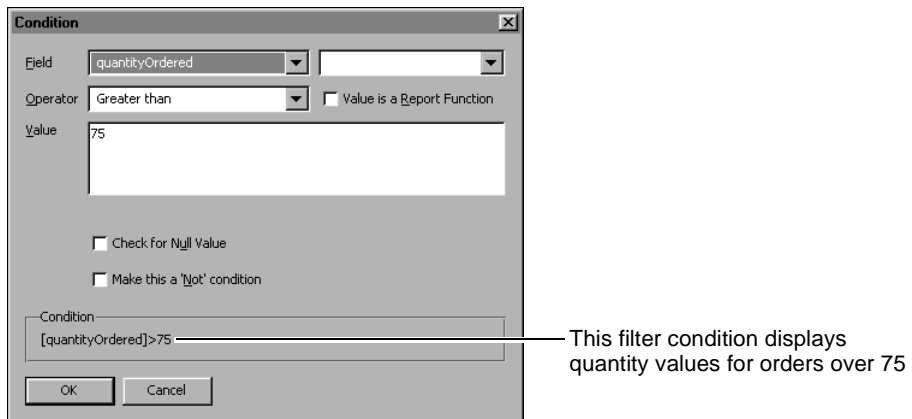
Figure 9-15 Creating a second filter condition
