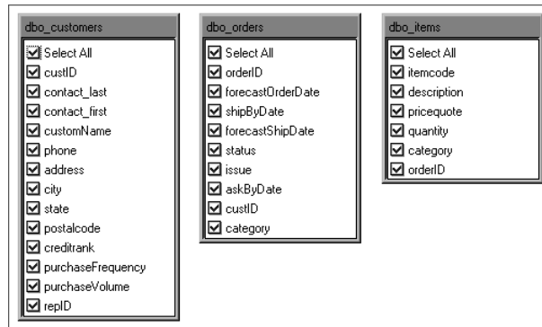
Figure 5-14 Selected information objects as they appear in Query Design
