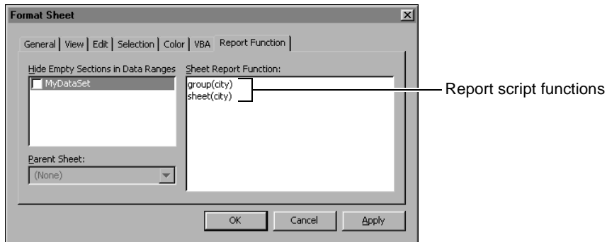
Figure 7-12 Using group and sheet report script functions
