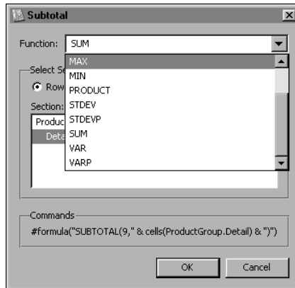
Figure 9-25 Selecting a SUBTOTAL function
