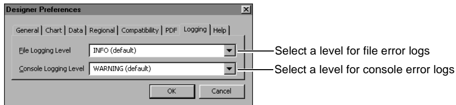
Figure 17-7 Setting error log level preferences
