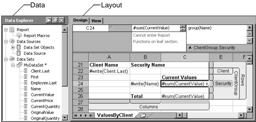
Figure G-21 Layout editor
