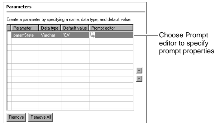
Figure 5-45 Choosing Prompt editor to specify a parameter's prompt properties
