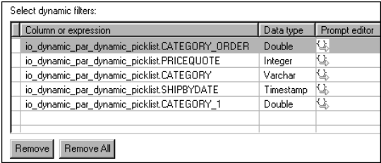
Figure 5-37 Selecting a dynamic filter
