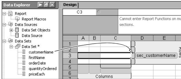
Figure 7-15 Creating a section and group from a data field
