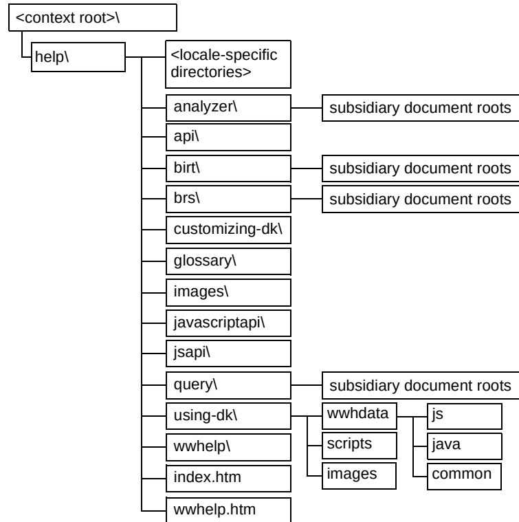
Figure 10-1 Java Component help directory structure
