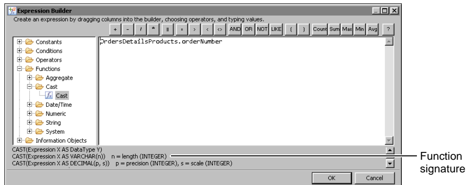
Figure 2-4 Using the expression builder to create expressions
