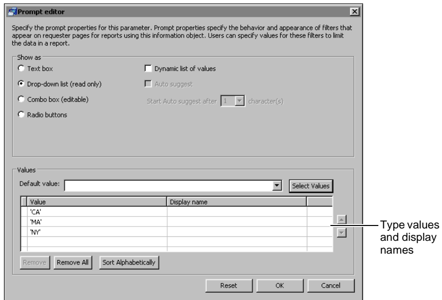
Figure 2-38 Typing a list of values and display names
