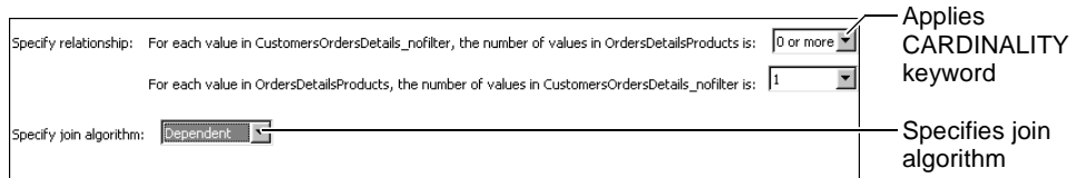
Figure 2-8 Optimizing a join
