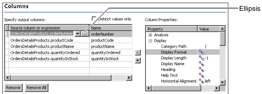
Figure 2-3 Defining output columns
