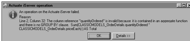
Figure 2-34 Information object query requires a GROUP BY clause
