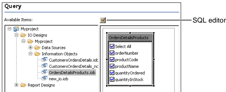
Figure 2-43 Opening the SQL text editor in Information Object Query Builder
