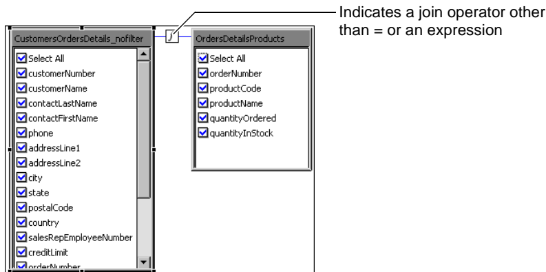
Figure 2-7 A join that uses an expression or an operator other than equality
