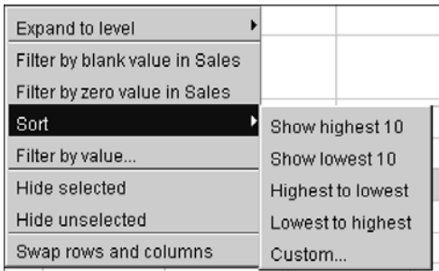
Figure 2-13 Sort options
