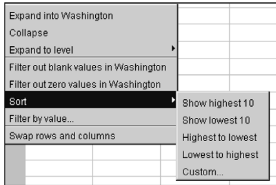
Figure 2-16 Sort options
